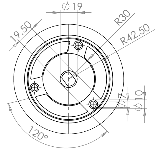
DETAIL A SCALE 2 : 5
